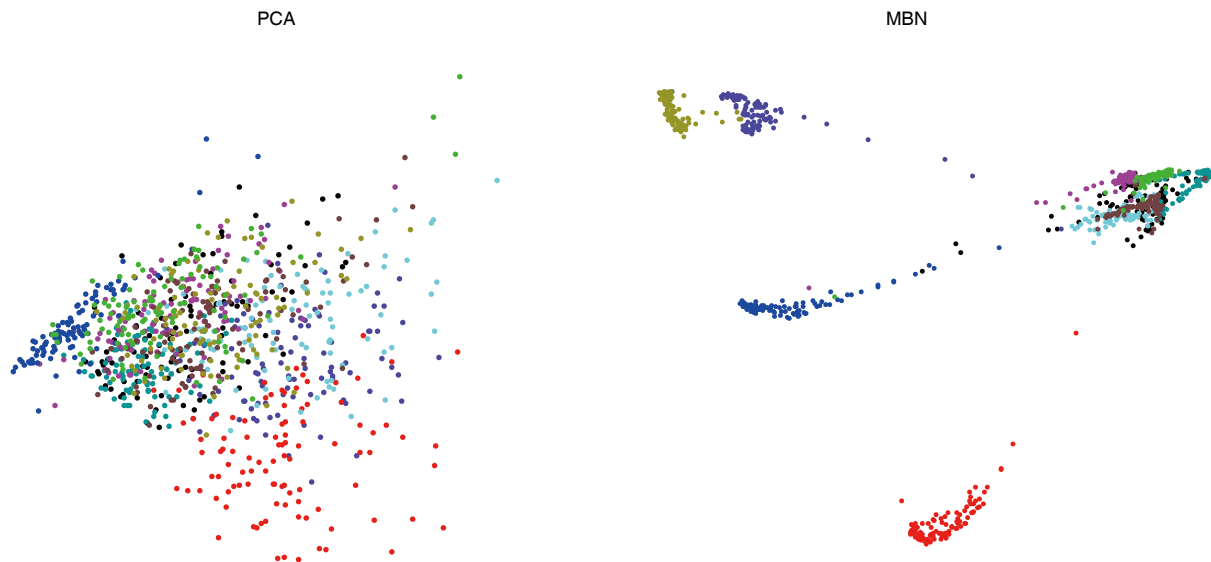
Fig. 1. Visualizations of 10 speakers by PCA and MBN respectively, where a 16-mixtures UBM with 0 EM iteration is used to produce their input supervectors. The speakers are labeled in different colors.
